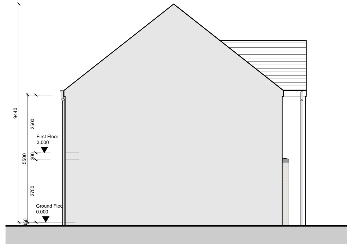
Side Elevation 01
