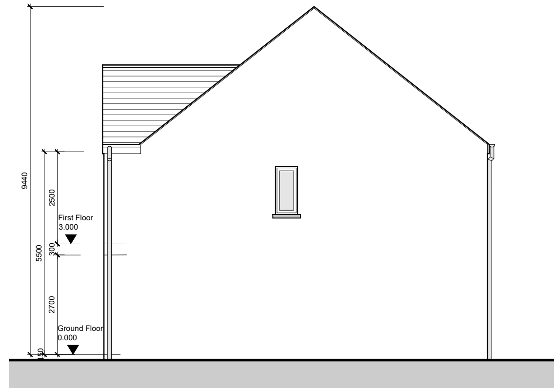
Side Elevation 02
